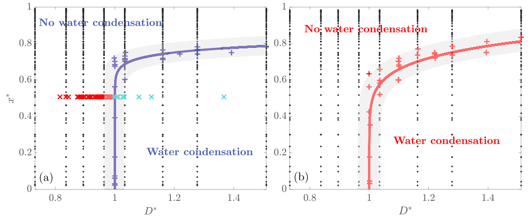
Figure 12. Condensation limits for different \text{H}_2\text{O} contents as a function of the dimensionless star-planet distance ( D^* , equation (13)) for a (a) grey radiative-convective and (b) nongrey k -correlated atmosphere. The plus signs correspond to the condensation limits obtained for different water contents and the cross markers stand for calculations made for different albedos and solar constants ranging respectively from 0.1 to 0.7 and from the young Sun's solar constant to the present-day value. Cross markers are blue if water condensation occurs and red if not. Parameters used for the calculations are given in Table 2.
