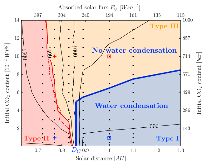
Figure 7. Surface temperature isotherms (black lines) and solidus temperature (red line) as a function of \text{CO}_2 content and solar distance at ERCS. Below water condensation limit (blue line), a water ocean can condense at the surface of the planet. Crosses and squares correspond to calculations shown on Figure 6. The different types of planet are represented by colored areas. The dashed lines stand for the limits obtained by considering a secular cooling only occurring over the liquid-state mantle (i.e., between the solidification front R_5 and the surface, see section 2.1.3 and Appendix B). Parameters used for the calculations are given in Table 2.
