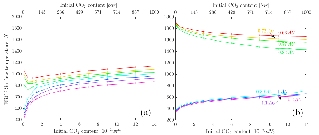
Figure 13. Surface temperatures obtained at ERCS for solar distances varying from 0.63 to 1.30 AU, initial \text{CO}_2 contents from 0.1 to 14 \times 10^{-2} wt % and initial water contents equal to (a) 0.031 M_{\text{EO}} and (b) 1.243 M_{\text{EO}} . Parameters used for the calculations are given in Table 2.
