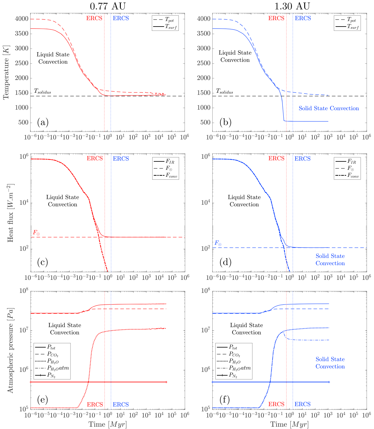
Figure 5. Thermal evolution of the magma ocean for two different distances from the Sun: 0.77 AU (a, c, and e, red) and 1.30 AU (b, d, and f, blue), grey atmosphere, without clouds, [H_2O]_0 = 0.621 M_{EO} , [CO_2]_0 = 5 \times 10^{-2} wt %. ERCS is indicated by the vertical dotted lines. P_{H_2Oatm} corresponds to the uncondensed H_2O partial pressure remaining in the atmosphere if condensation occurs at surface and stores water in the oceans (here a 480 m deep water ocean is formed at 1.30 AU). Corresponding thermal atmospheric profiles at ERCS are shown in Figure 4. Parameters used for the calculations are given in Table 2.
