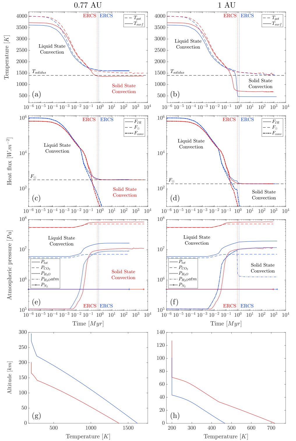
Figure 6. Thermal evolution of the magma ocean for two different initial \text{CO}_2 contents: 10^{-2} (blue curves) and 10^{-1} wt % (red curves), and two different solar ocean distances: 0.77 AU (a, c, e, and g, crosses in Figures 7 and 8) and 1 AU (b, d, f, and h, squares in Figures 7 and 8), grey radiative-convective atmosphere, without clouds, [\text{H}_2\text{O}]_{t_0} = 0.621 M_{\text{EO}} . At ERCS, for D = 0.77 AU, P_{\text{H}_2\text{O}}/P_{\text{CO}_2} = 1.17 for [\text{CO}_2]_{t_0} = 10^{-2} wt % and P_{\text{H}_2\text{O}}/P_{\text{CO}_2} = 0.13 for [\text{CO}_2]_{t_0} = 10^{-1} wt %. For D = 1 AU, P_{\text{H}_2\text{O}}/P_{\text{CO}_2} = 0.19 for [\text{CO}_2]_{t_0} = 10^{-2} wt % and P_{\text{H}_2\text{O}}/P_{\text{CO}_2} = 0.145 for [\text{CO}_2]_{t_0} = 10^{-1} wt %. At 1 AU, for [\text{H}_2\text{O}]_{t_0} = 0.621 M_{\text{EO}} and [\text{CO}_2]_{t_0} = 10^{-2} wt %, a 910 m deep water ocean is formed at ERCS. Parameters used for the calculations are given in Table 2.
